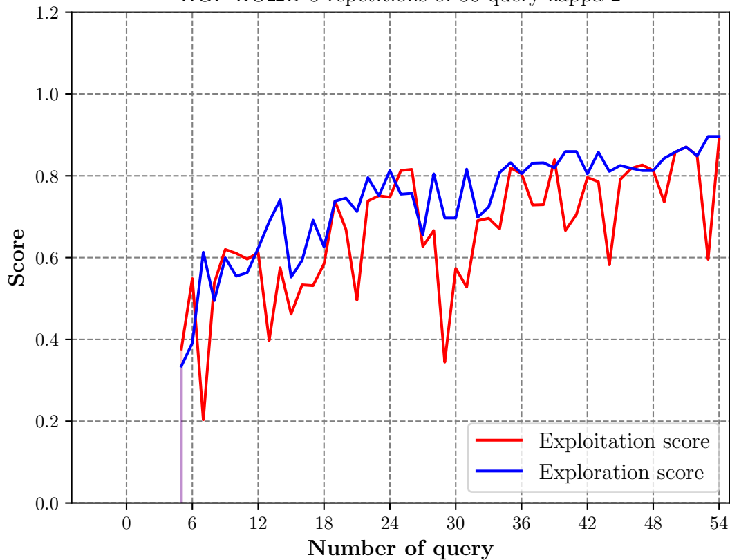
HGP-BO_2D 5 repetitions of 50 query kappa 2
